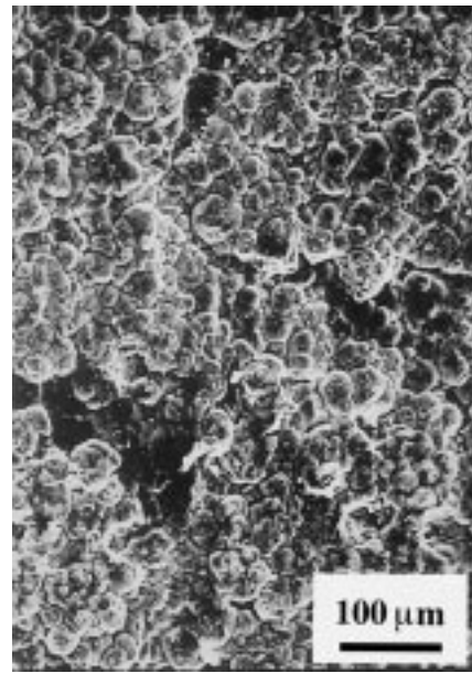
Fig. 9. SEM photomicrograph of composite surface morphology; \phi_{\text{PS}} = 0.054 , c_{\text{CPC}}^* = 0.2 \text{ mol kg}^{-1} ; j = 500 \text{ A m}^{-2} \omega = 100 \text{ s}^{-1} .
