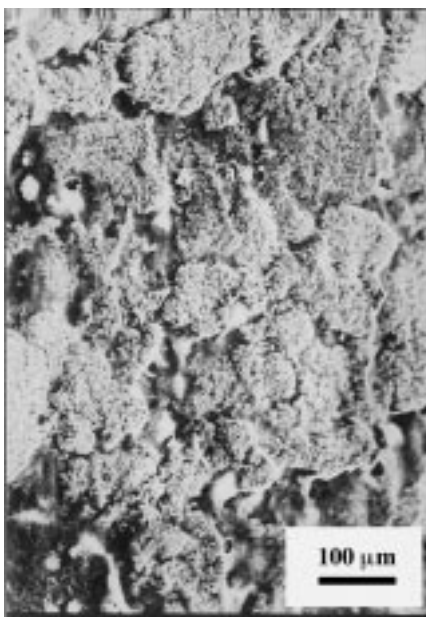
Fig. 8. SEM photomicrograph of composite surface morphology; \phi_{\text{PS}} = 0.054 , \omega = 100 \text{ s}^{-1} and c_{\text{CPC}}^* = 0.02 \text{ mol kg}^{-1} ; j = 50 \text{ A m}^{-2} .
