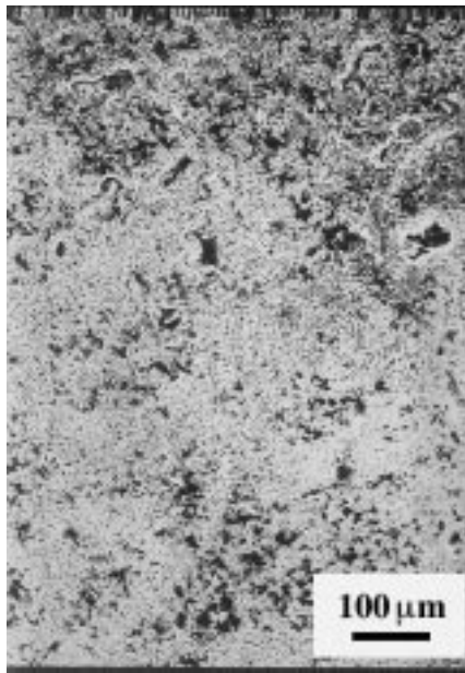
Fig. 7. SEM photomicrograph of composite surface morphology; \phi_{\text{PS}} = 0.047 , \omega = 100 \text{ s}^{-1} and c_{\text{CPC}}^* = 0.02 \text{ mol kg}^{-1} ; j = 500 \text{ A m}^{-2} .
